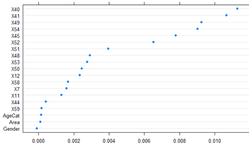
Figure 5. Conditional variable importance in the item-based model of the data ( R^2 = 0.664 )
