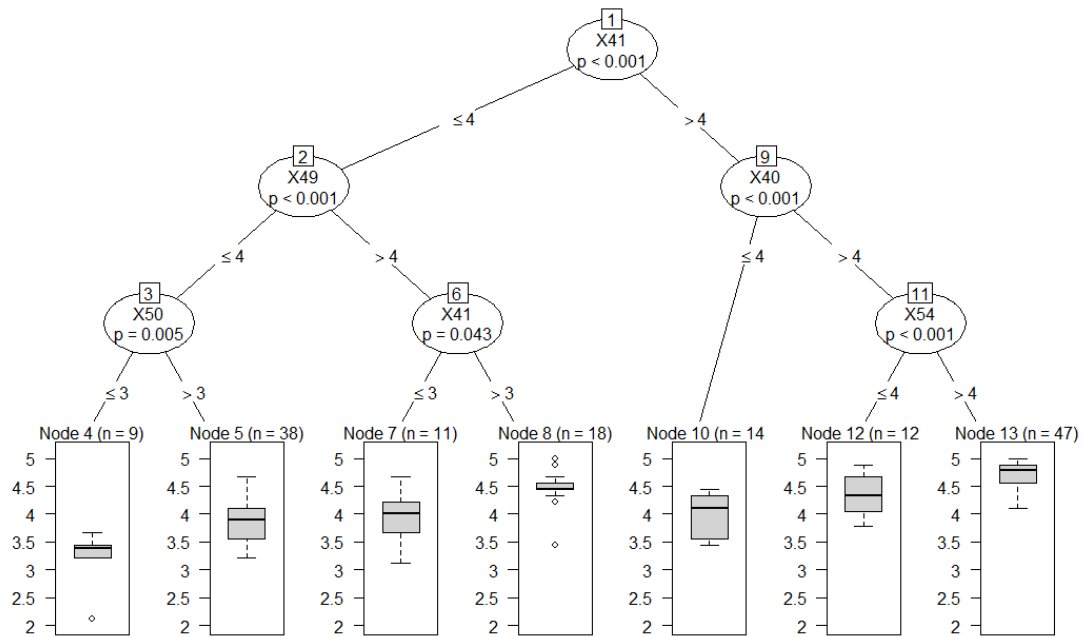
Figure 4. CIT for the item-based model of the data ( R^2 = 0.615 )
