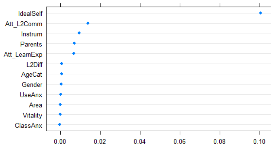
Figure 3. Conditional variable importance in the scale-based model of the data ( R^2 = 0.686 )
